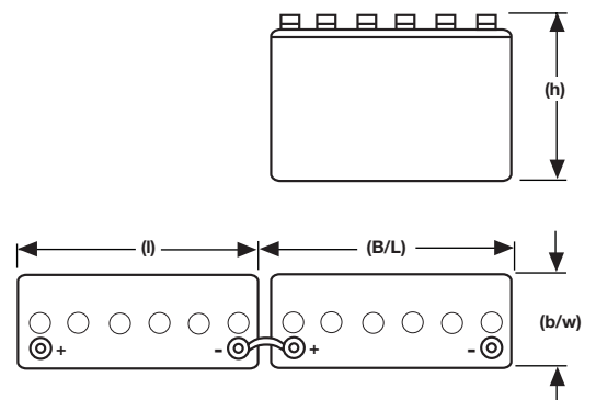
12 V Block
