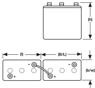
6 V Block
